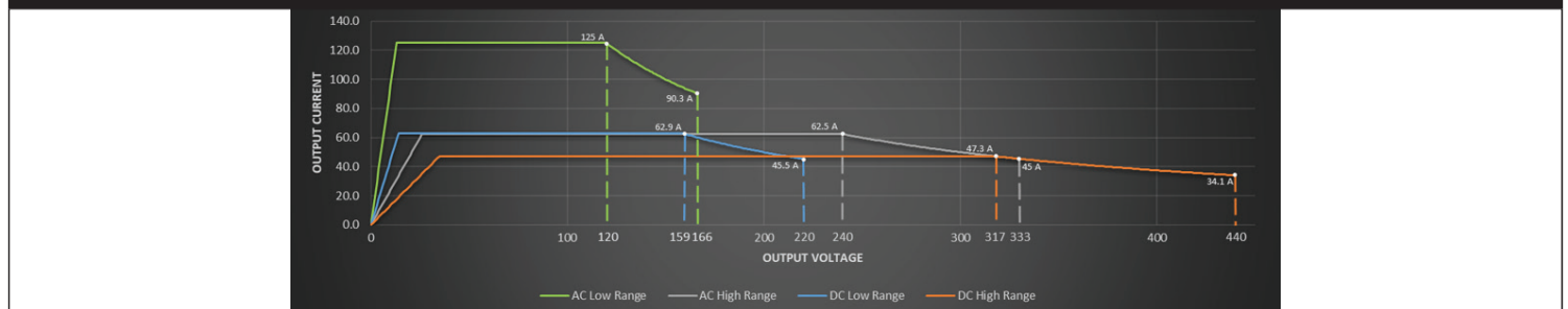
CONSTANT POWER MODE - AVAILABLE MAX AC OR DC CURRENT VS. PROGRAMMED VOLTAGE
